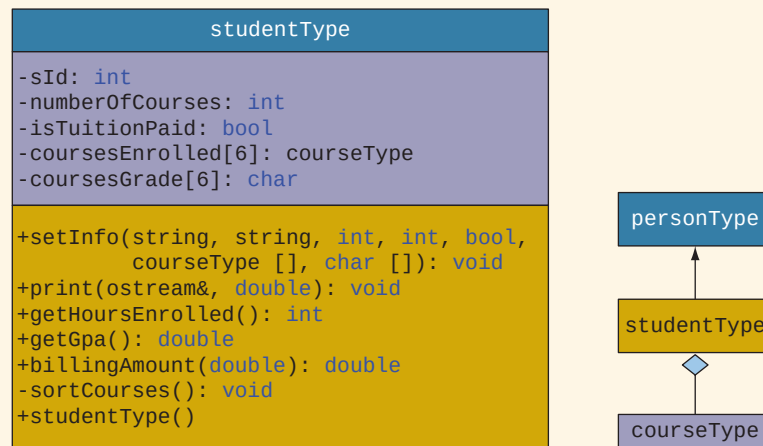
FIGURE 12-10 UML class diagram of the class studentType together with inheritance and composition (aggregation) relation
