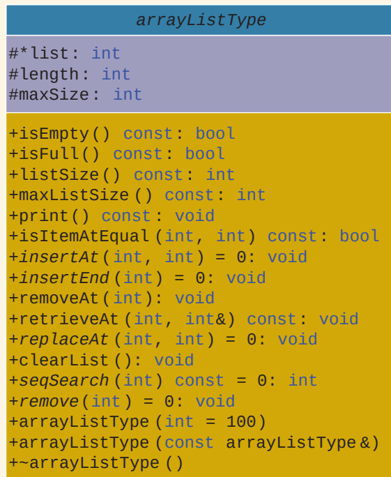
FIGURE 13-22 UML diagram of the class arrayListType
