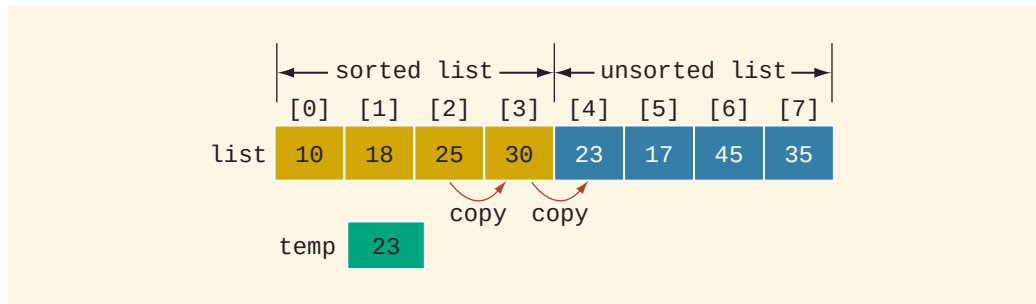
FIGURE 19-18 List before copying list[3] into list[4] and then list[2] into list[3]
