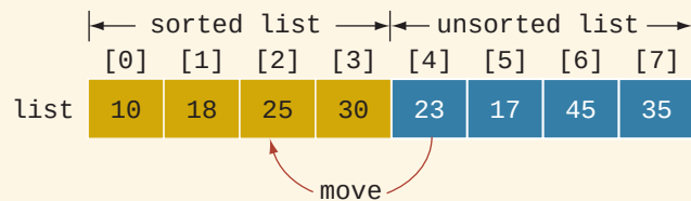
FIGURE 19-16 Move list[4] into list[2]
