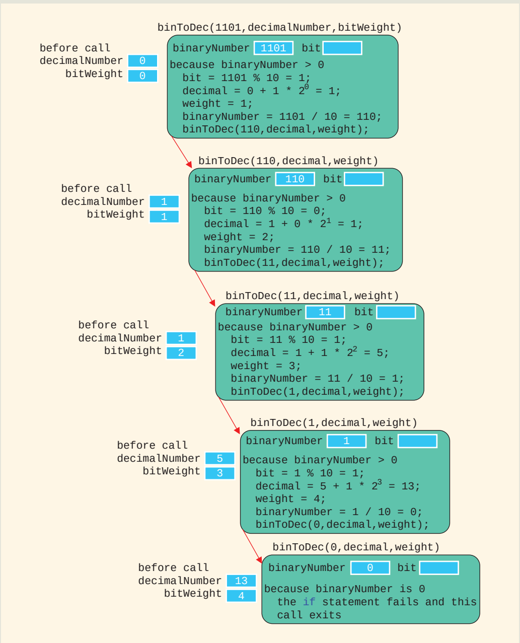
FIGURE 16-8 Execution of binToDec(1101, decimalNumber, bitWeight);
