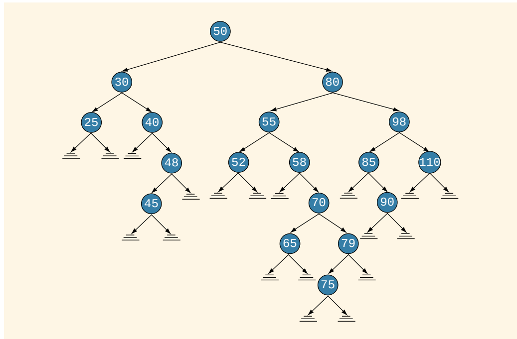
FIGURE 20-14 Figure for Exercises 9 to 13
