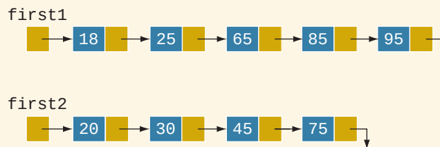
FIGURE 19-38 Sublists before merging
