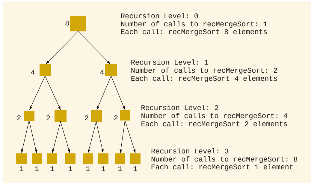
FIGURE 19-41 Levels of recursion to recMergeSort for a list of length 8
