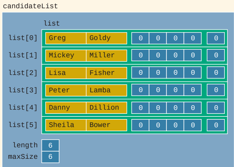
FIGURE 19-45 Object candidateList after a call to the function fillNames
