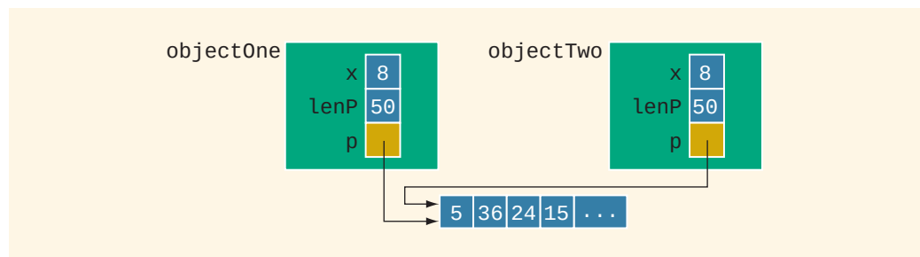
FIGURE 13-16 Objects objectOne and objectTwo after the statement objectTwo = objectOne; executes
