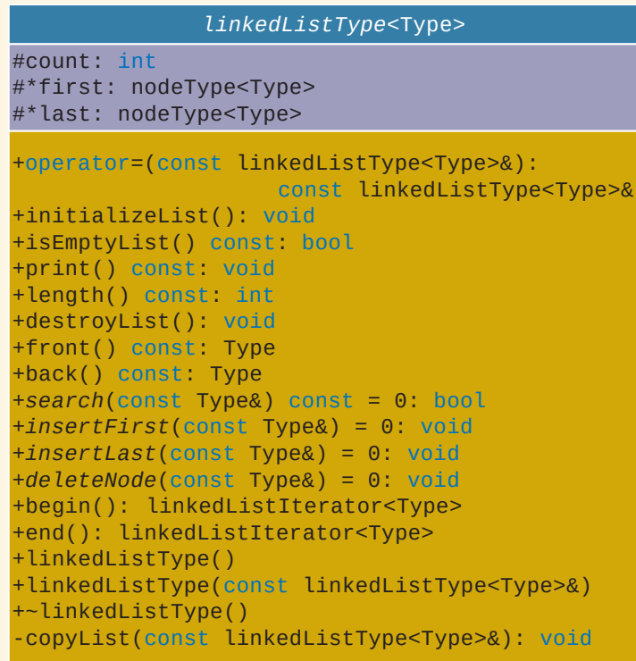
FIGURE 17-20 UML class diagram of the class linkedListType
