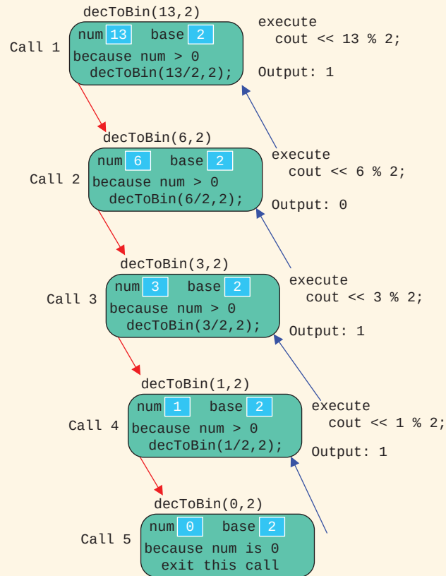
FIGURE 16-9 Execution of decToBin(13, 2)
