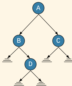
FIGURE 20-6 Binary tree for an inorder traversal
