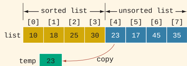
FIGURE 19-17 Copy list[4] into temp
