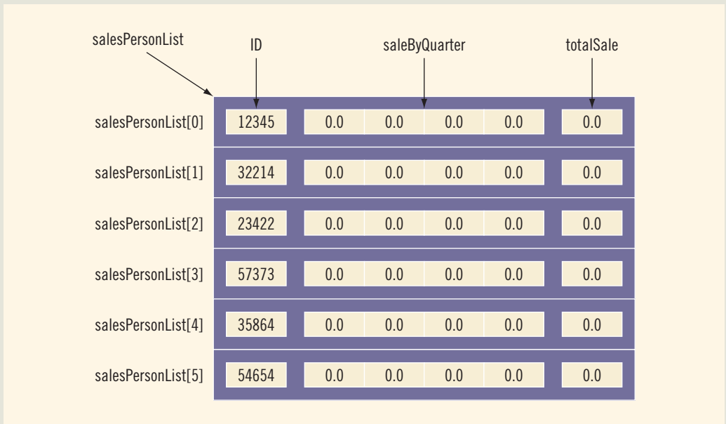
FIGURE 10-10 Array salesPersonList after initialization
