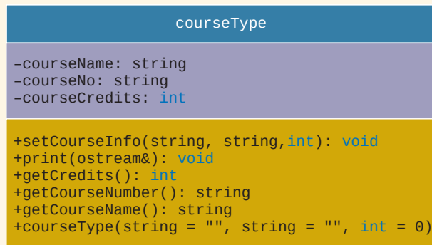
FIGURE 12-9 UML class diagram of the class courseType
