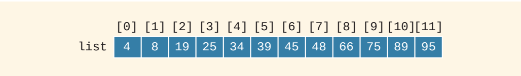
FIGURE 19-4 Sorted list for a binary search
