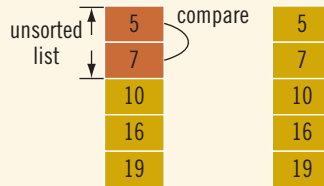
FIGURE 19-10 Elements of list during the fourth iteration
