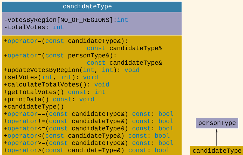
FIGURE 19-42 UML class diagram of class candidateType
