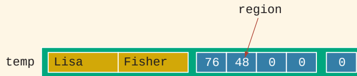
FIGURE 19-49 Object temp after temp.updateVotesByRegion(region, votes); executes
