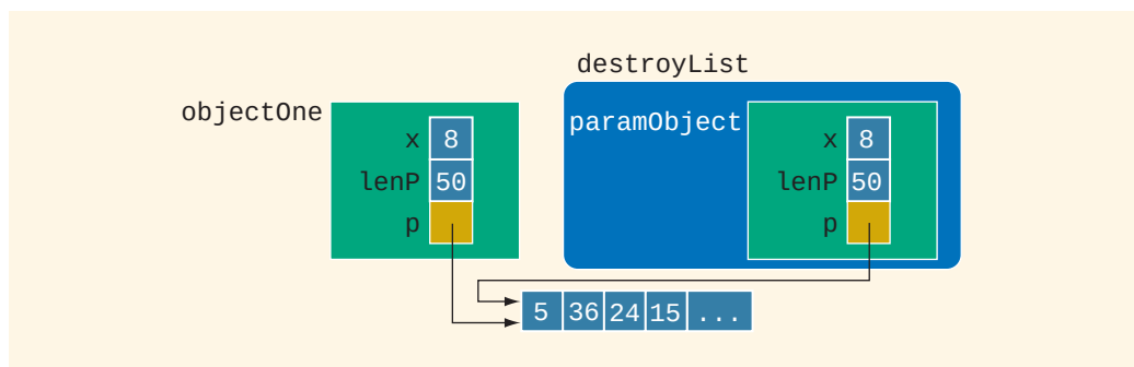
FIGURE 13-20 Pointer member variables of objects objectOne and paramObject pointing to the same array
