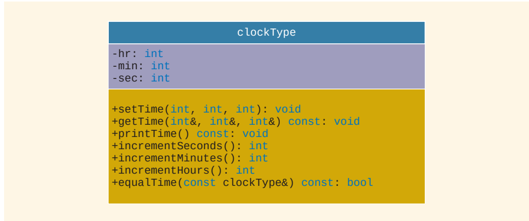
FIGURE 11-1 UML class diagram of the clockType class
