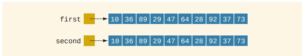
FIGURE 13-12 first and second both pointing to their own data
